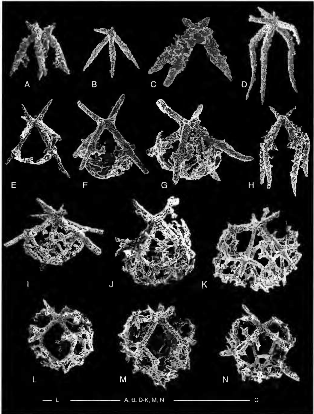
FIG. 8. — A-C, Archaeosemantis brevispinosa Kamata n. sp., A, holotype, DEUY-YK3617; B, paratype, DEUY-YK3627; C, paratype, DEUY-YK3618; D, H, A. cristianensis Dumitrica; D, DEUY-YK3629; H, DEUY-YK3481; E-G, I-N, Parentactinia nakatsugawaensis Sashida; E, DEUY-YK3538; F, DEUY-YK3479; G, DEUY-YK3545; I, DEUY-YK3509; J, DEUY-YK3603; K, DEUY-YK3486; L, DEUY-YK3506; M, DEUY-YK3588; N, DEUY-YK3422. Scale bars: 100 \mu m.
